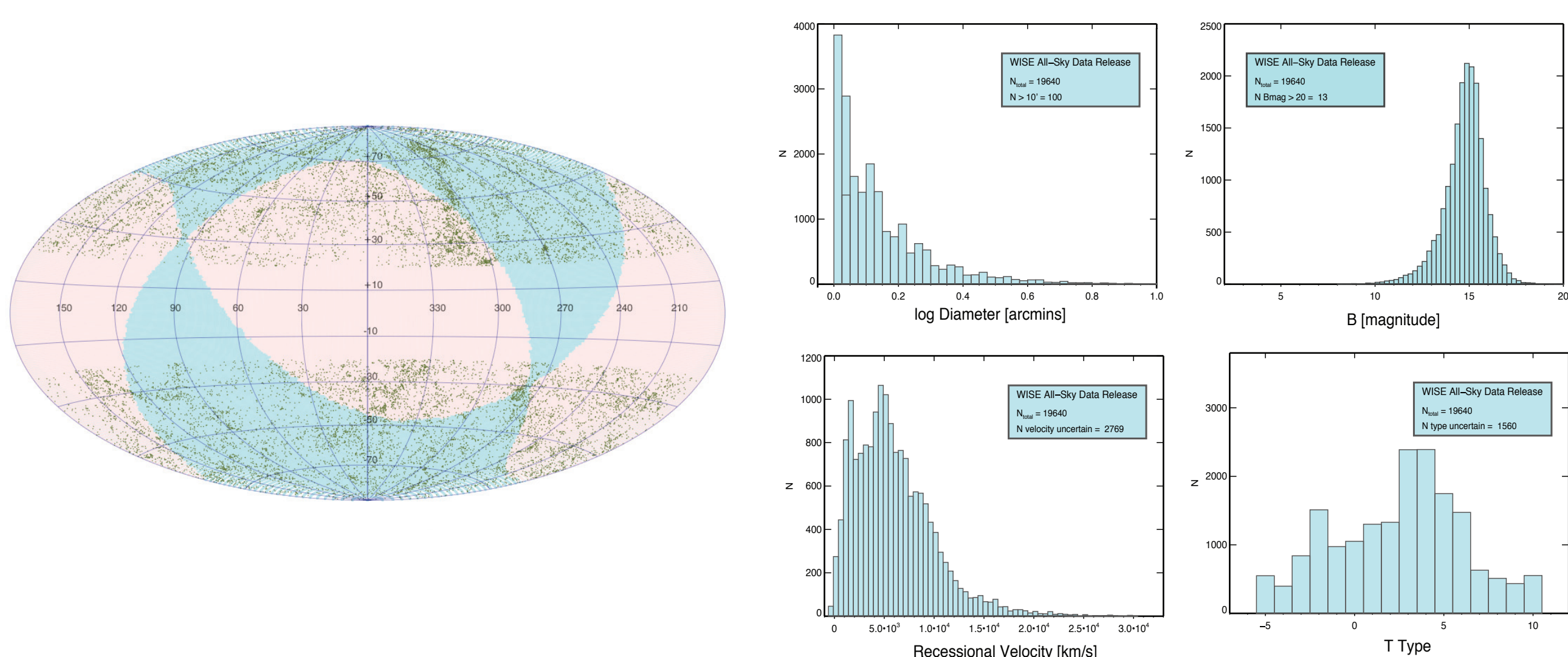
Figure 2: Sample spatial distribution in Galactic coordinates. The red region indicates the WISE preliminary data release footprint. The blue region represents the remaining sky coverage to be included in the final WISE data release.
