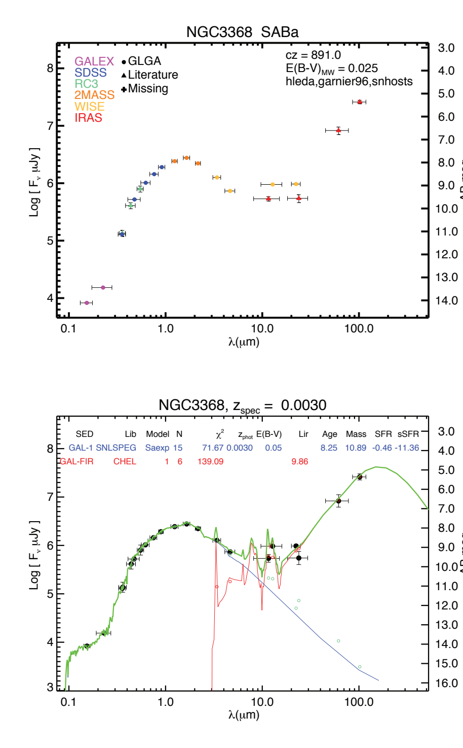
Figure 6: SED fitting of WNGA photometry.
