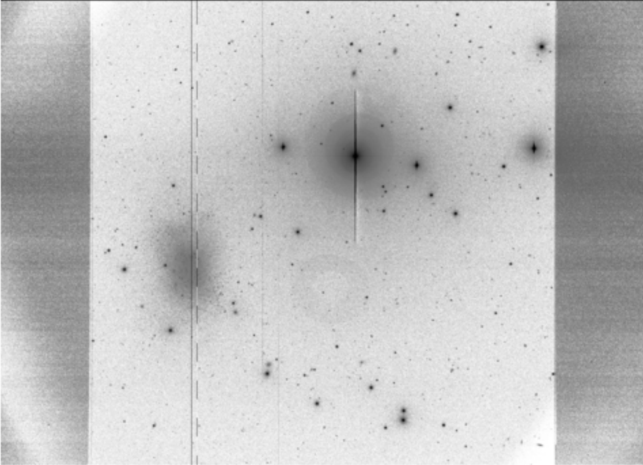
SextansB VIS 2014 12 20 21
