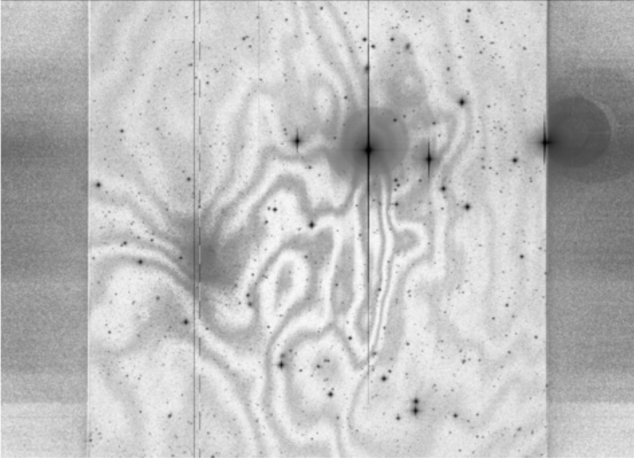
SextansB VIS 2014 12 19 20
