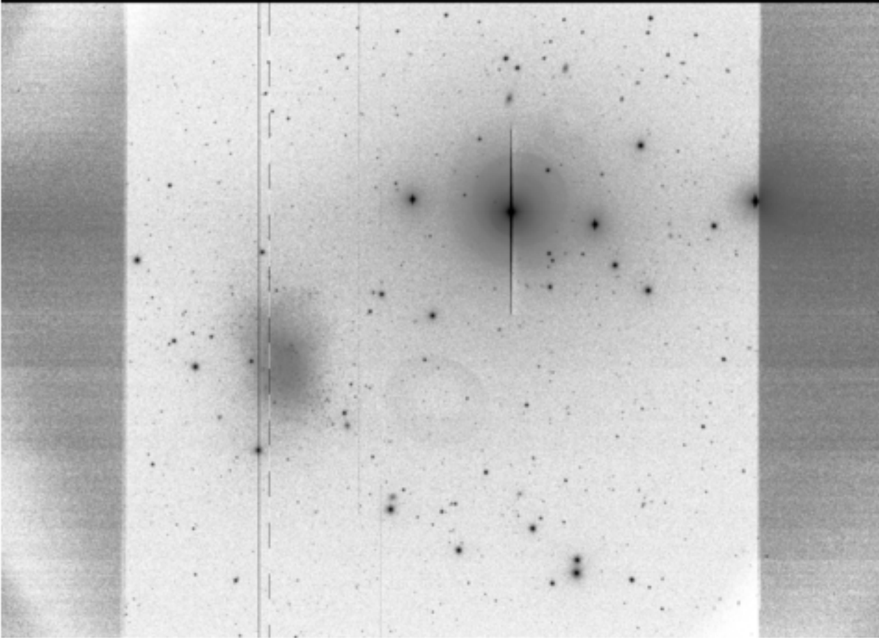
SextansB VIS 2014 12 18 19
