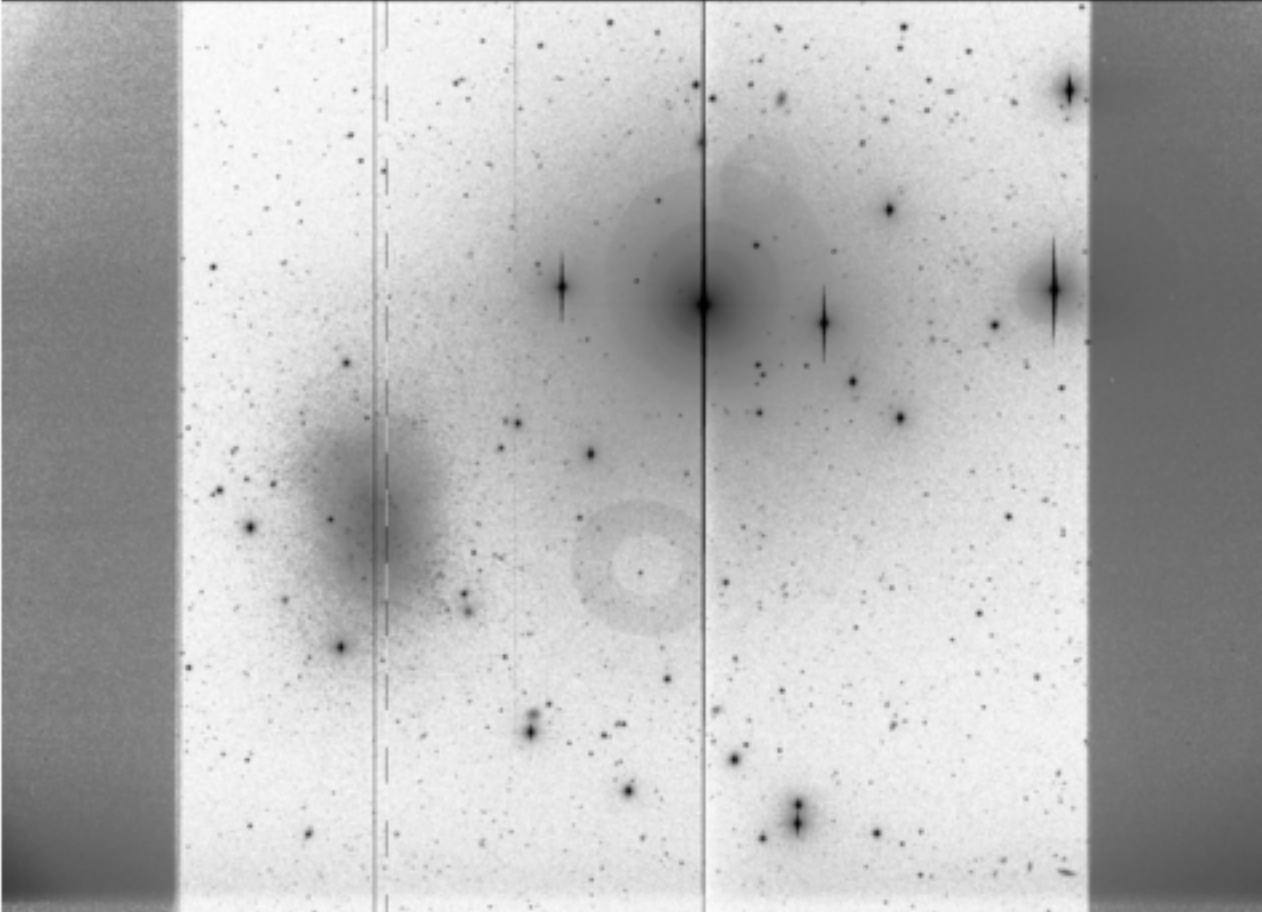
SextansB VIS 2014 12 21 22
