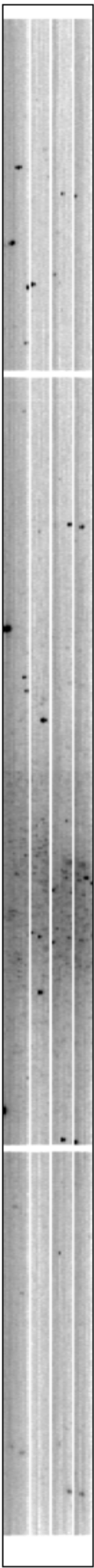
SextansB VIS 2014 12 18 19
