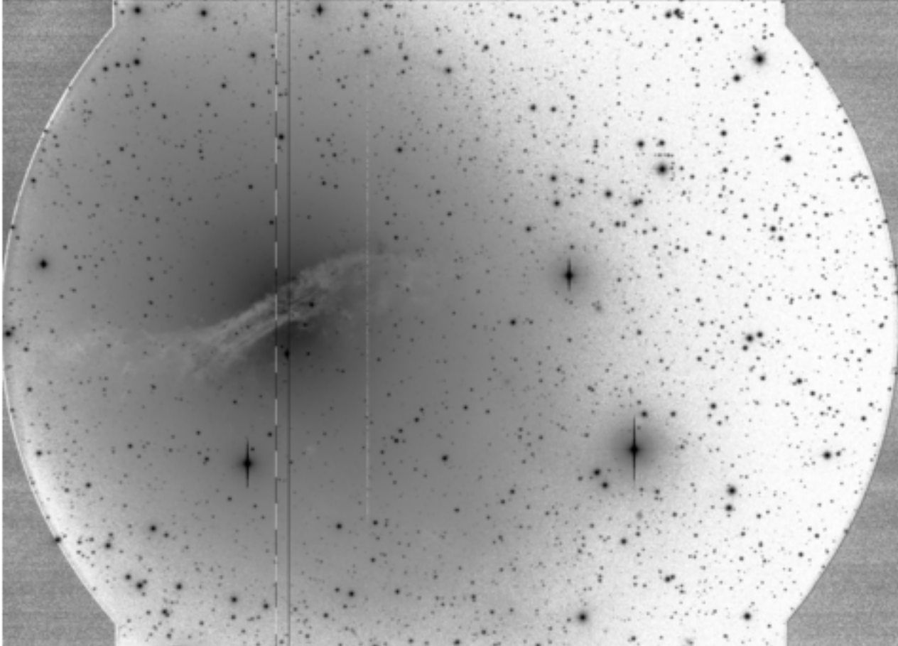
N5128_VIS_2013_06_01_02
