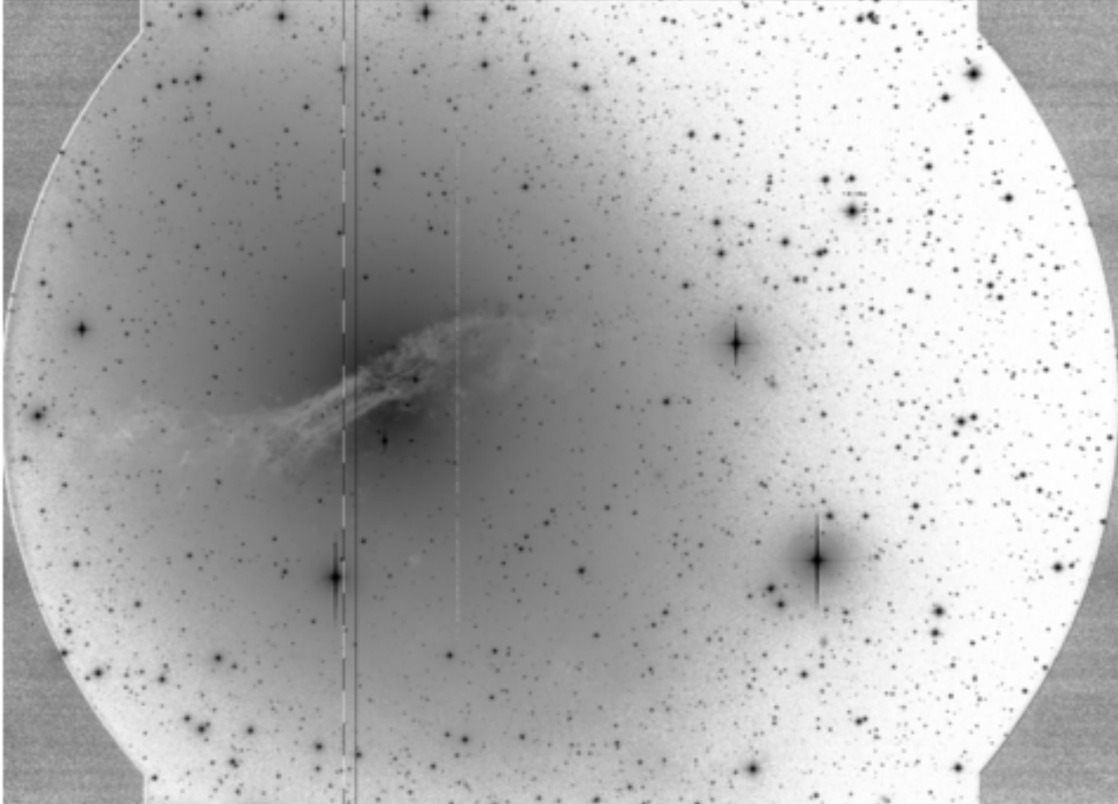
N5128_VIS_2013_06_03_04
