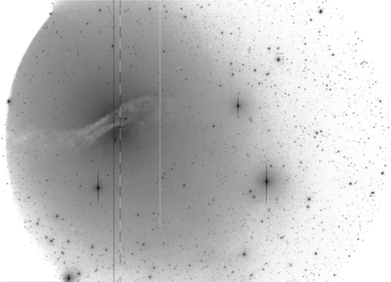
N5128_VIS_2011_02_28_01
