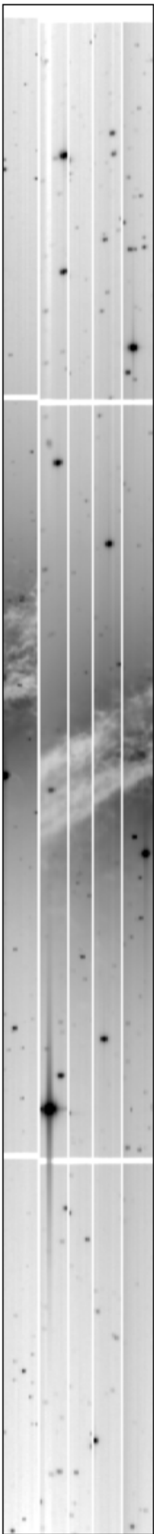
N5128_VIS_2011_02_28_01
