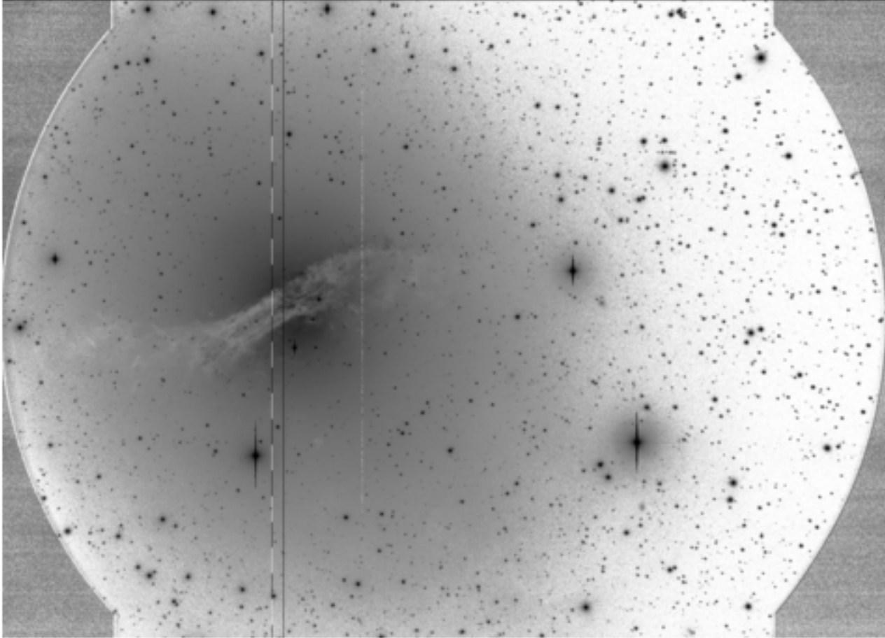
N5128_VIS_2013_06_02_03
