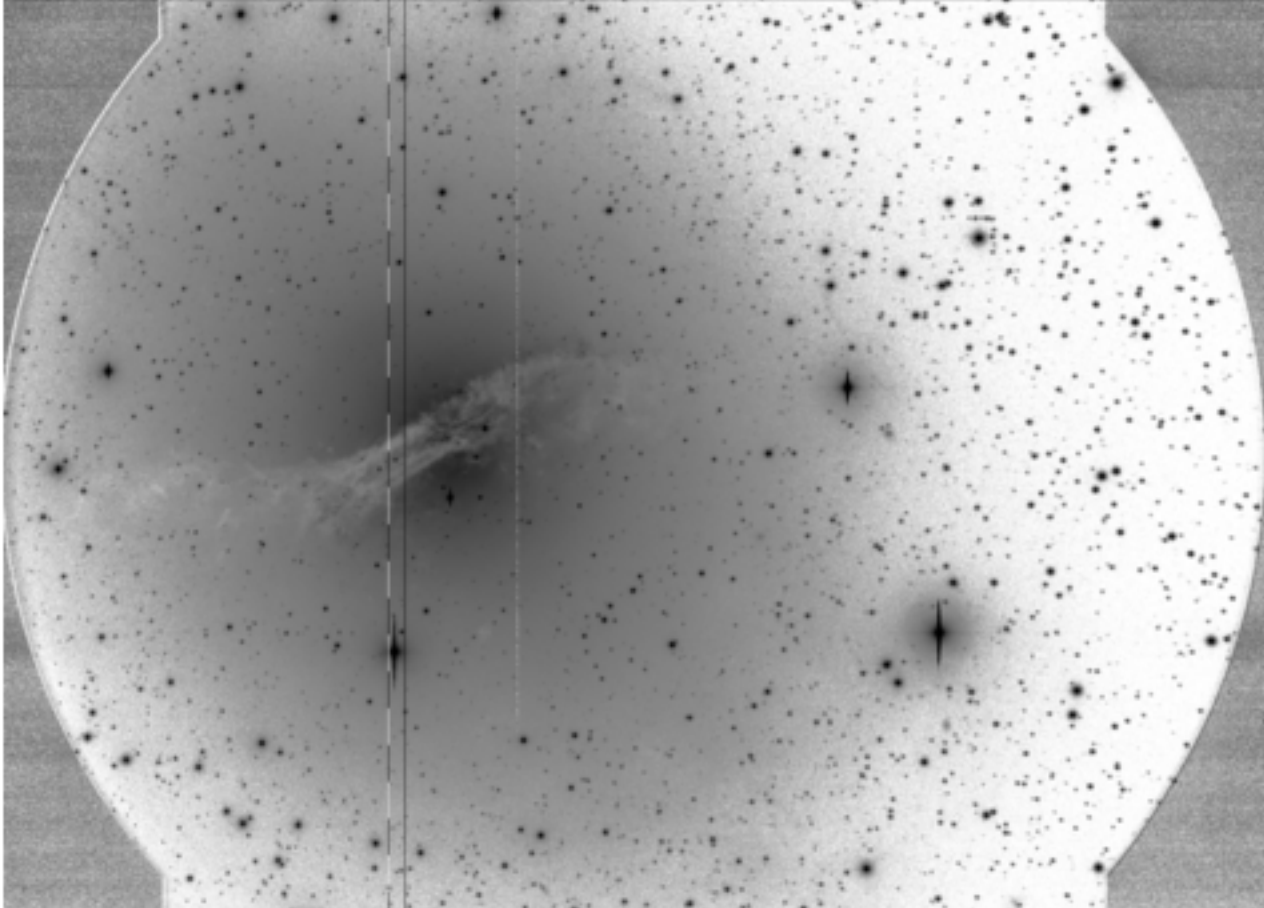
N5128_VIS_2013_06_04_05
