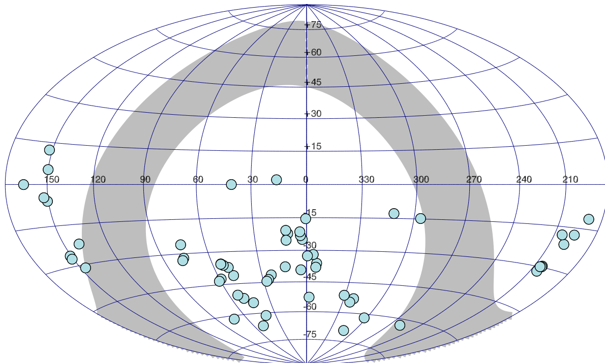
Equatorial Coordinate Projection
