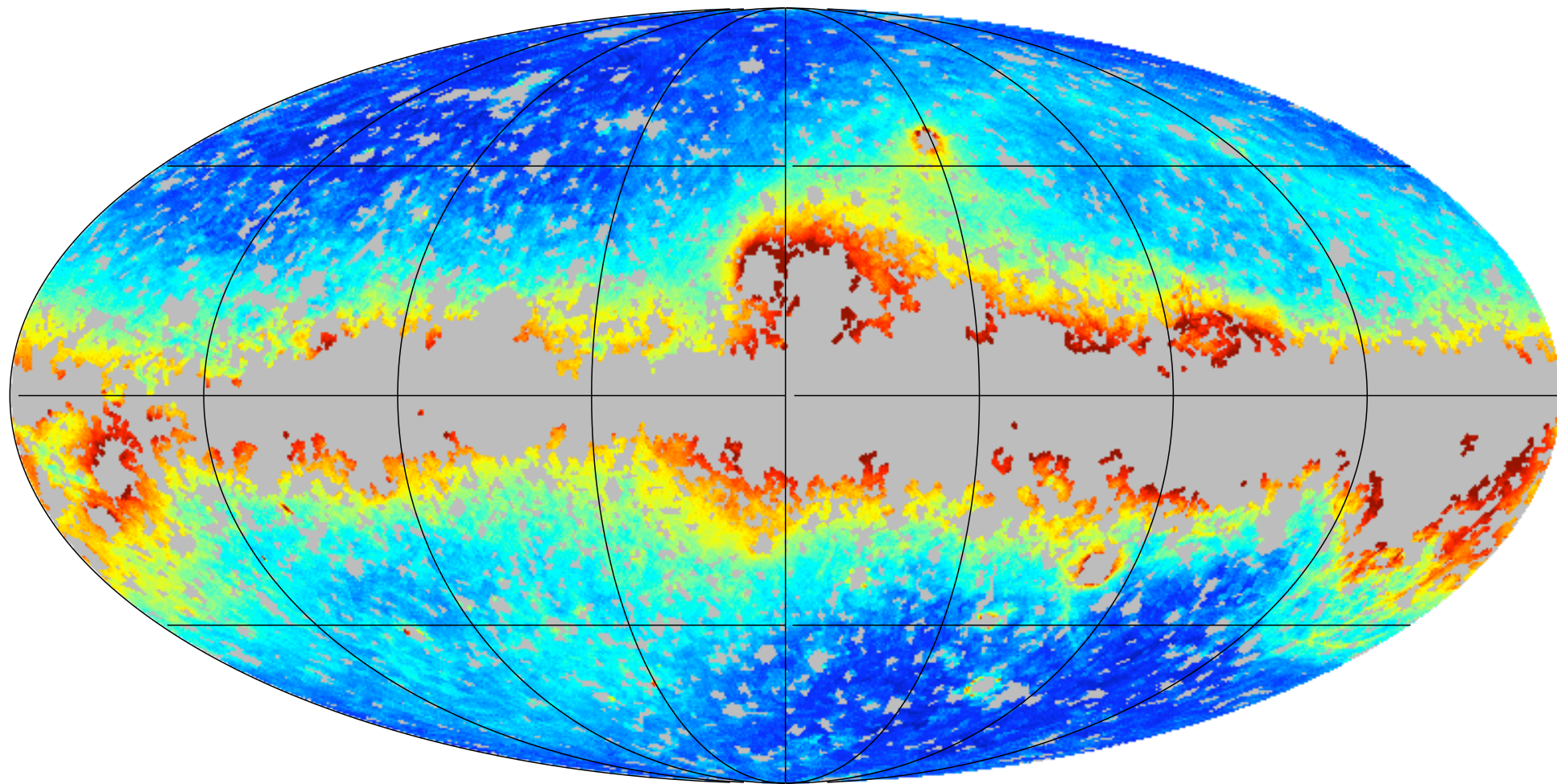
NUV sky (Galactic)
