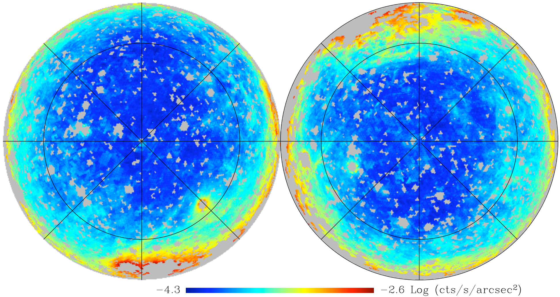
FUV sky (Galactic)
