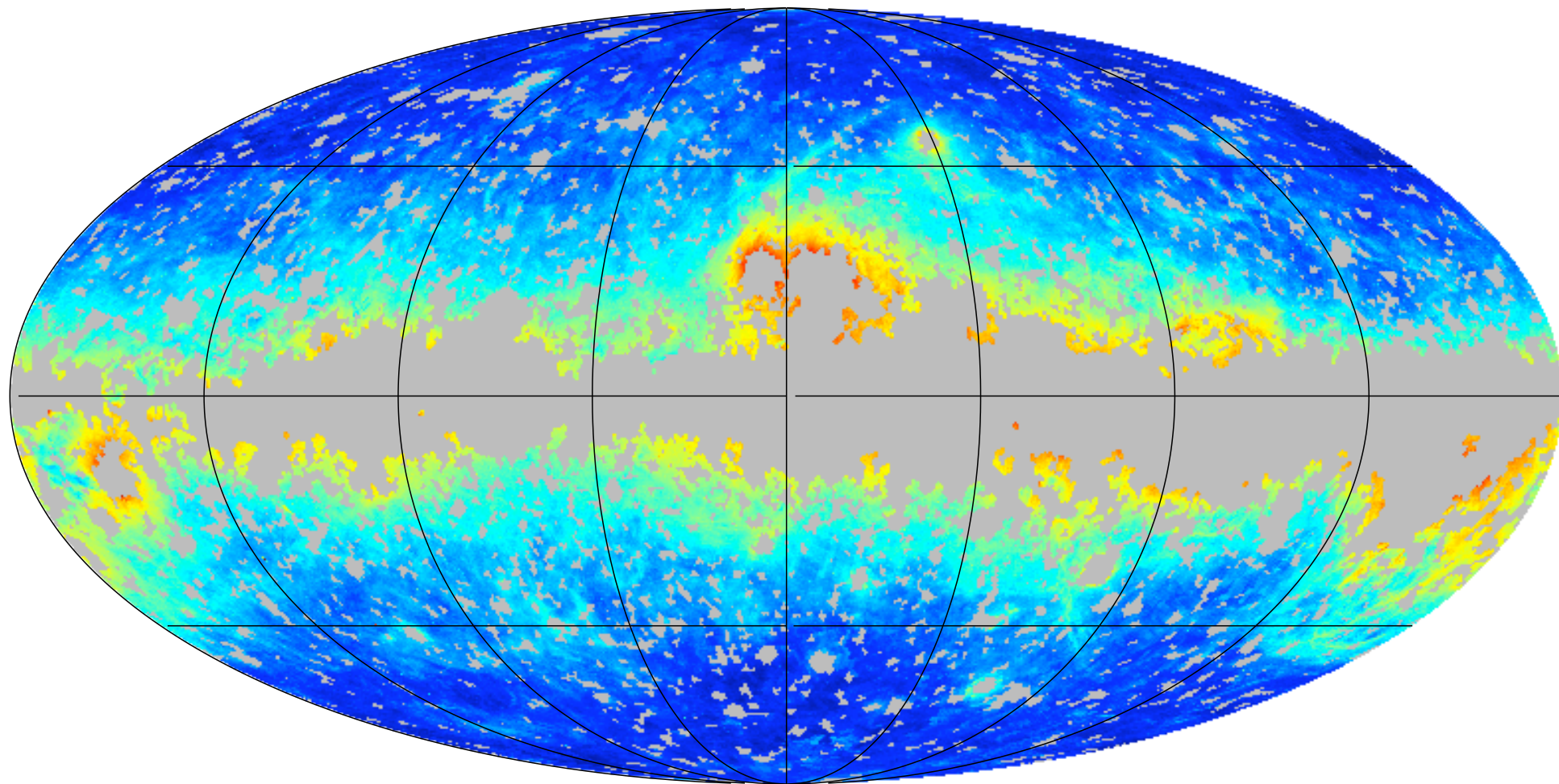
FUV sky (Galactic)
