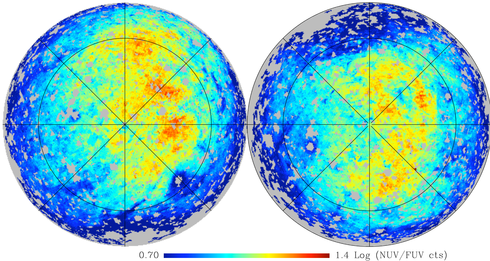
UV sky color (Galactic)
