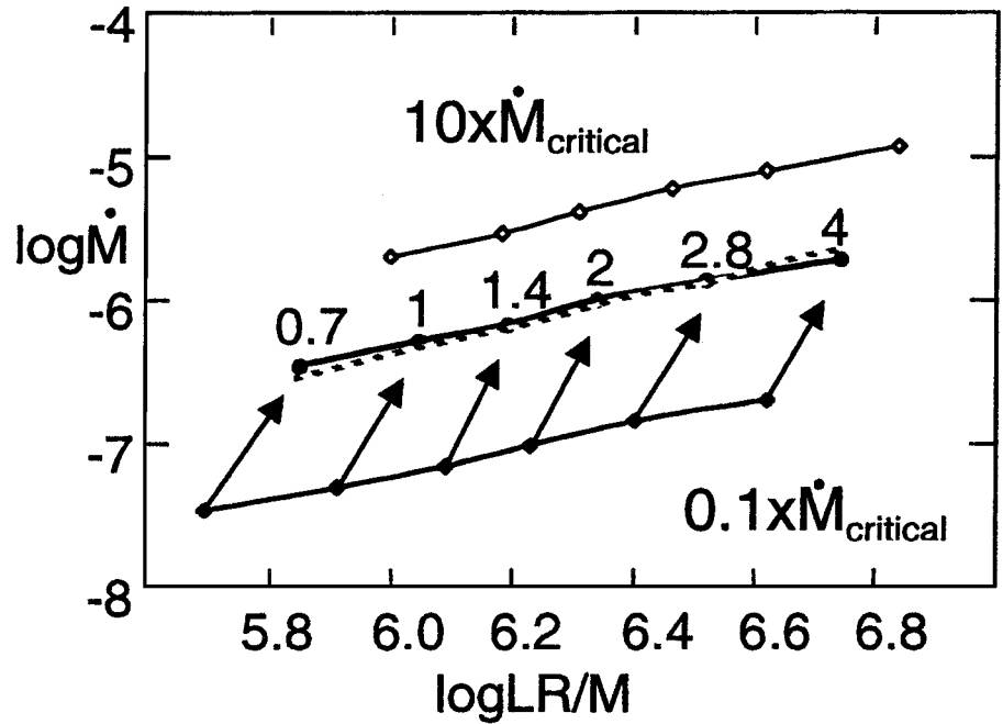
Figure 8 Mass loss rate versus LR/M for the “cliff” stars and mass loss rates 1/10, 10 times the “cliff” rates. Reimers (1975) relation is seen to coincide almost exactly with the “cliff” position. Thus Reimers’ relation tells us the properties of stars when they are losing mass, not how any one star loses mass over time.
