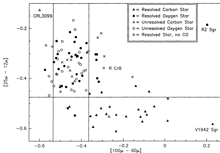
FIG. 5.—An IRAS two-color diagram is shown for all extended objects (filled symbols), including those beyond 500 pc, along with objects within 500 pc which were not found by the MFP to be extended (open symbols). No color corrections have been applied to the fluxes from the PSC. Not shown are two planetary nebulae with very blue [25 - 12] colors, NGC 6720 and NGC 2346. IRAS 09372 + 1212, Y Hya, and IRC - 10139 are not shown because of problems with one or more of the IRAS fluxes for these objects.
