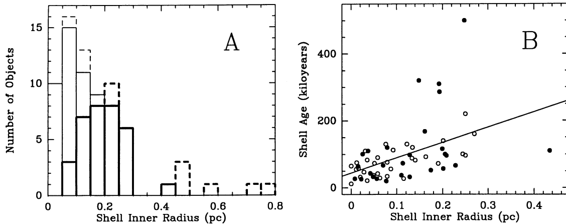
FIG. 4.—(a) A histogram of the inner shell radii is shown. The bold line histogram shows the values for those shells whose inner radii had an angular size of 1' or more, and may have actually been resolved. The thin line histogram shows the values for objects whose fitted inner radii are smaller than the IRAS 60\ \mu\text{m} diffraction limit, and probably have little or no physical significance. Solid lines are used for the objects which have been detected in CO, while a dashed line is used for objects with published nondetections. For the stars with CO emission, the radii are distributed rather uniformly through the range of 0.05–0.25 pc and only PQ Cep has an inner radius larger than 0.3 pc. (b) The calculated age of the dust shells for 59 of the stars in Table 1, plotted as a function of the inner shell radius. Carbon stars are plotted as filled circles; oxygen-rich objects are unfilled. NGC 6720 and the stars without CO detections were not included in this plot because their ages were not calculated. Also shown is the least-squares best-fit line. The weak correlation is stronger for the carbon-rich envelopes.
