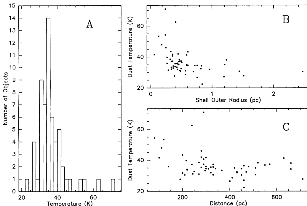
FIG. 6.—(a) Histogram of calculated dust temperatures. Four of the shells, those of R Leo (53 K), W Hya (54 K), R CrB (63 K), and U Hya (71 K) seem to be significantly warmer than average. (b) Distribution of calculated shell temperatures as a function of the shells' outer radii. Note that the warmest shells are much smaller than average, therefore the average temperature of the dust should be higher. (c) Calculated shell temperatures as a function of distance. All of the warmest shells are also closer than average, allowing material nearer the star to be resolved.
