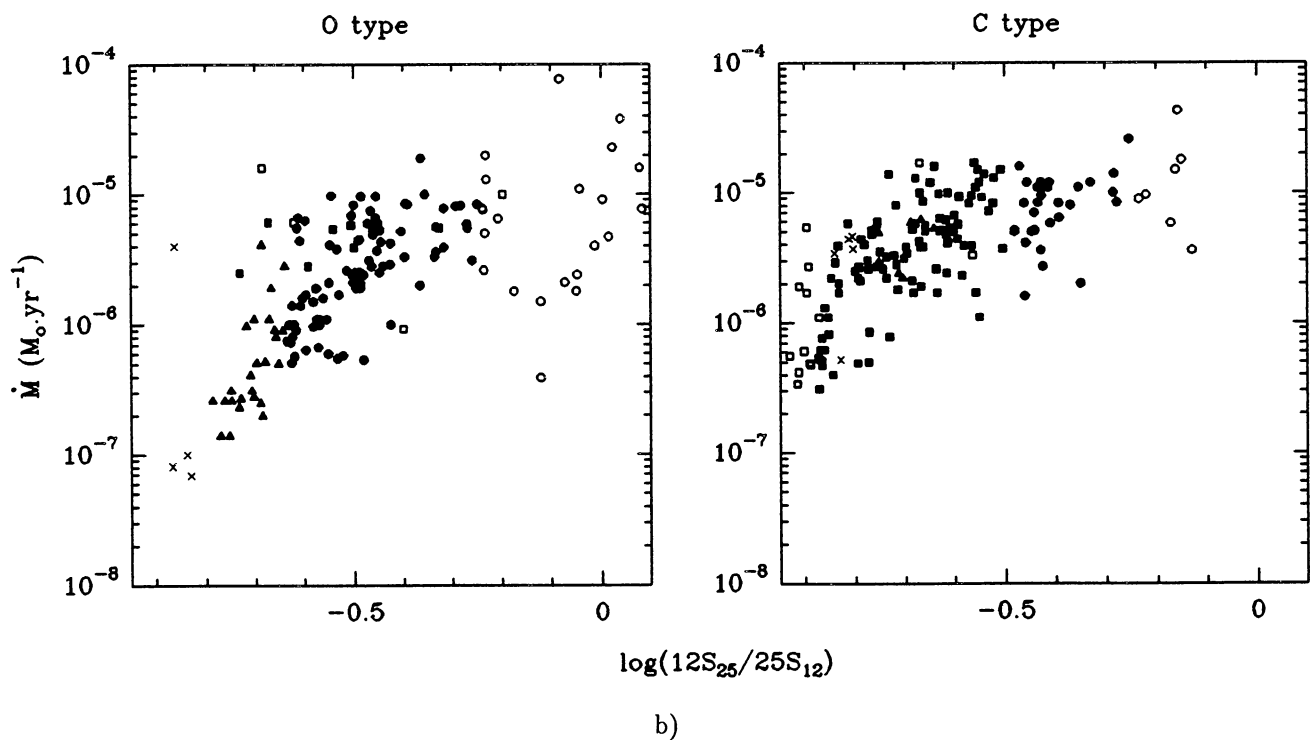
Fig. 9a,b. Correlation between mass loss rates and IRAS properties. In Fig. 9a, \dot{M} was calculated assuming R_{CO} = 3 \cdot 10^{17} cm (Eq. 3 in Sect. 4). In Fig. 9b, \dot{M} and R_{CO} were consistently calculated (Eqs. 6). Symbols are defined in the Fig. 6 caption
