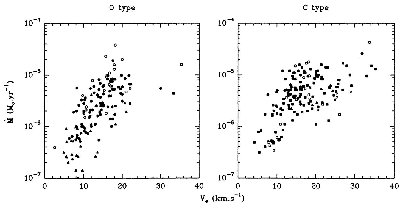
Fig. 8. Correlation between the expansion velocity and the mass loss rate derived from Eqs. (6) for O- and C-rich AGB stars. Symbols are defined in the Fig. 6 caption
