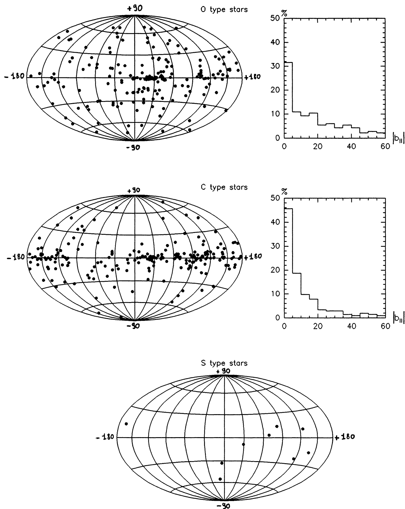
Fig. 4. Galactic distributions of the CO-HCN sample displayed on an Aitoff projection centered on the galactic center for the three chemical types (O, C, S). We also present latitude histograms for O- and C-rich sources
