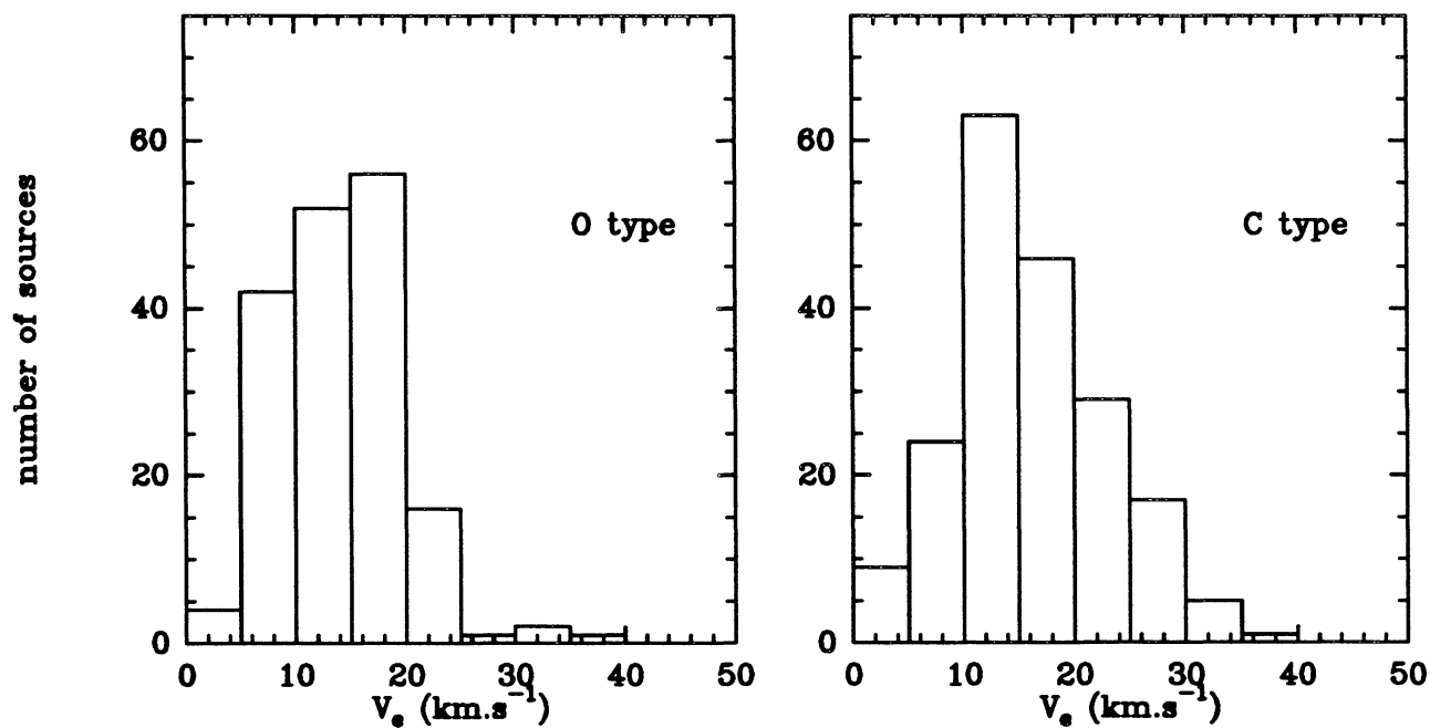
Fig. 7. Expansion velocity histograms. M supergiants and post-AGB stars are removed
