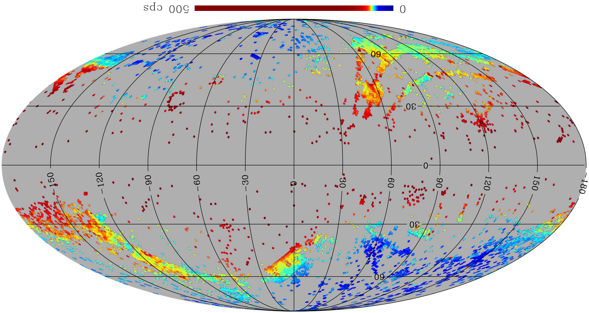
MSC NUV SKYBG (Galactic)
