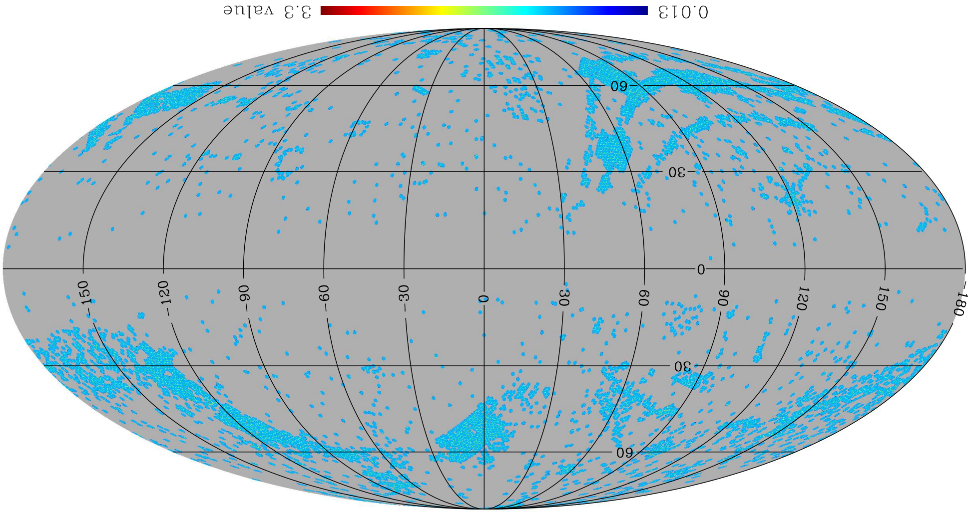
MSC NUV COVRAC (Galactic)
