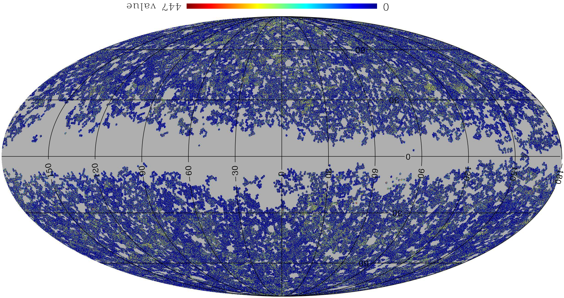
ASC NUV FLAGMAP (Galactic)
