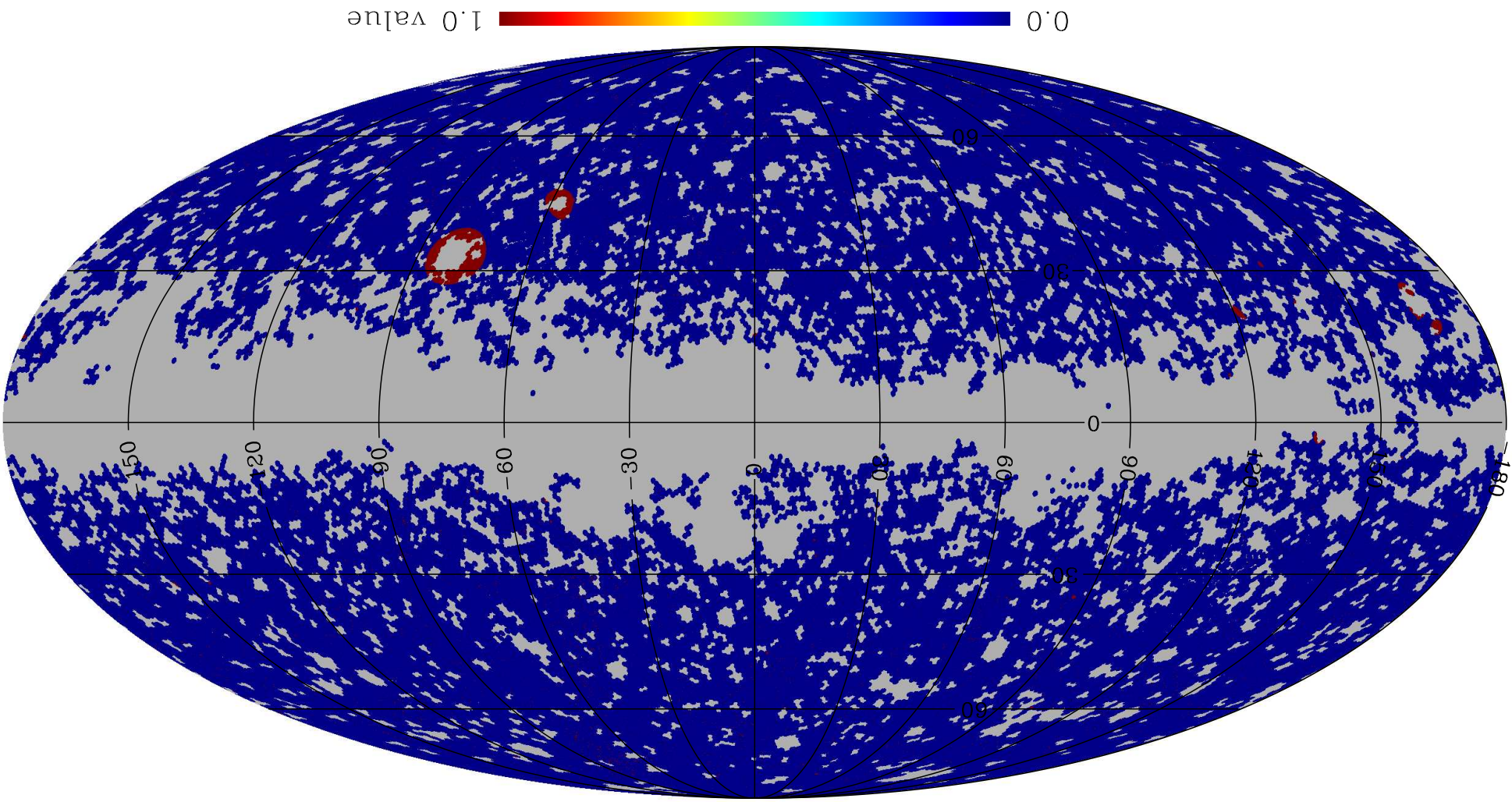
ASC NUV EXT-FLAGMAP (Galactic)
