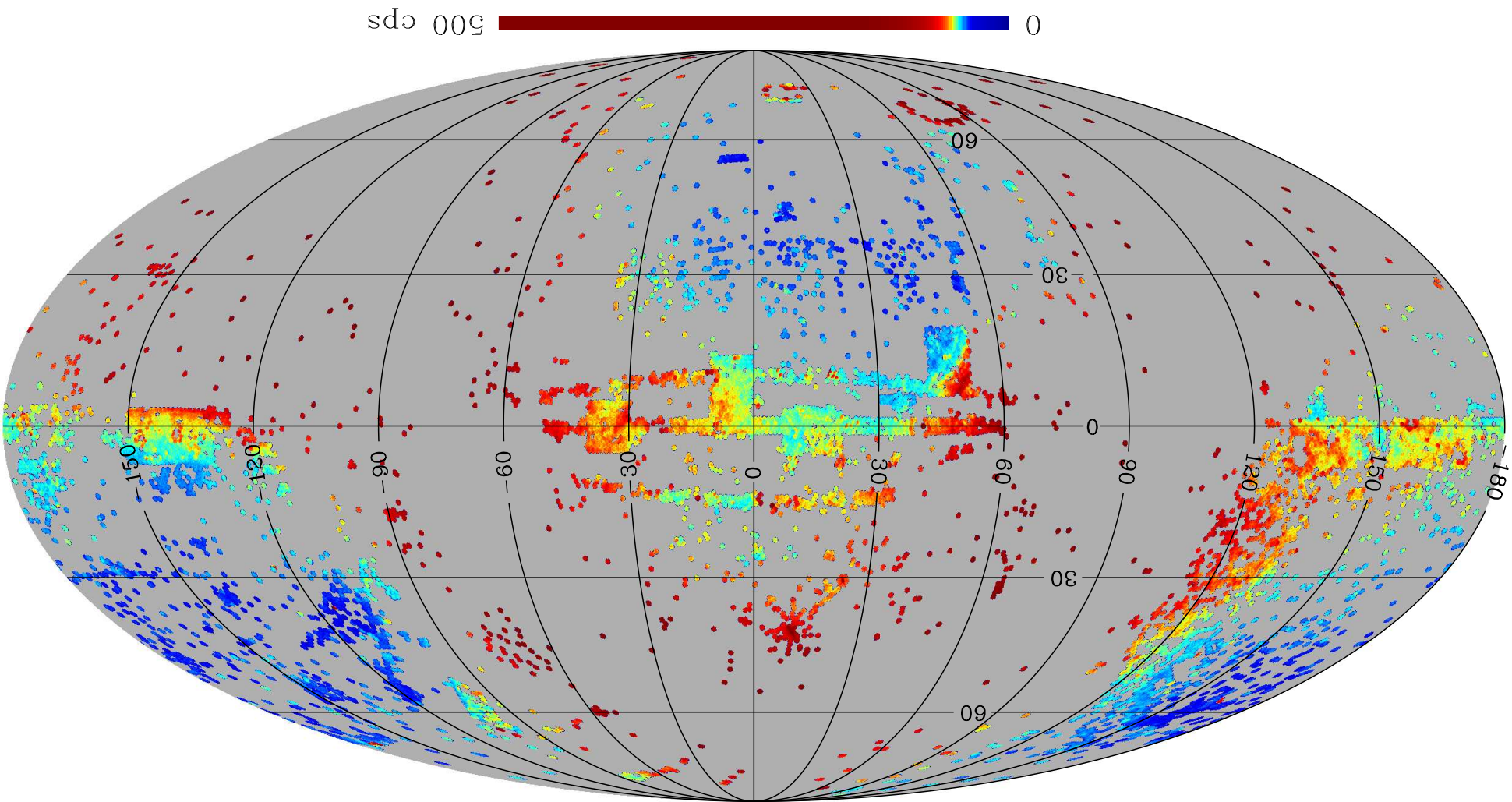
MSC NUV SKYBG (Equatorial)
