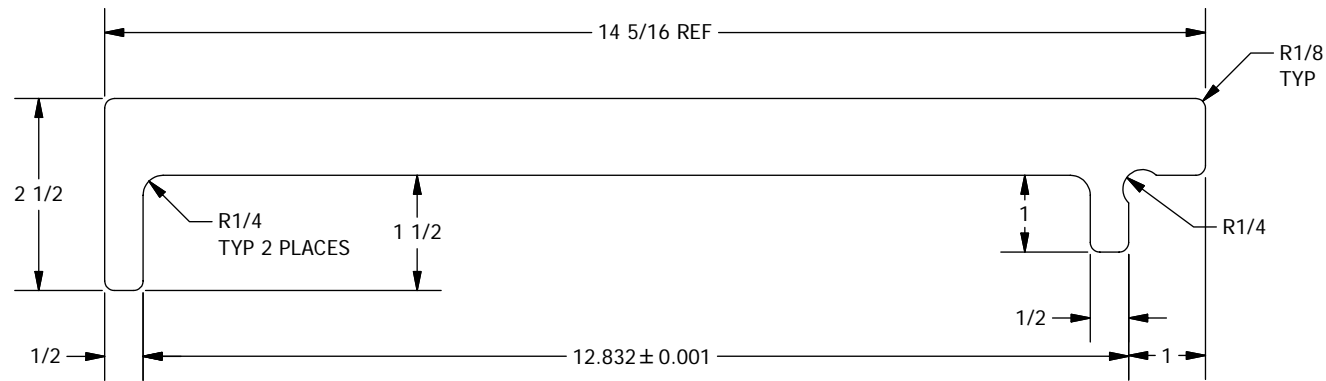
PFS14018 Dewar to PFS5 Spacing Gauge
