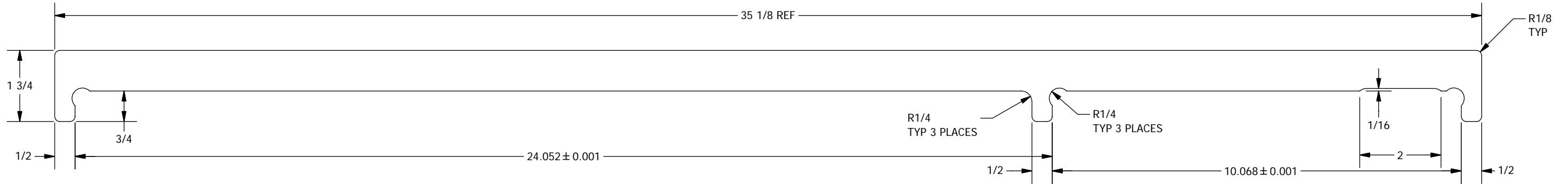
PFS14019 Camera/Collimator Lens Spacing Gauge
