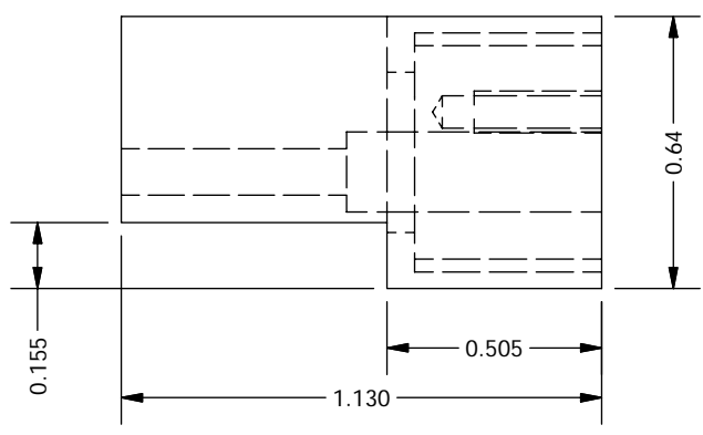
VIEW B-B
