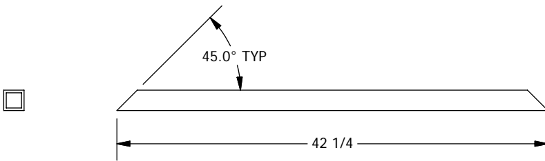
PFS03017 Insulation Frame Horizontal Short Quantity: 4
