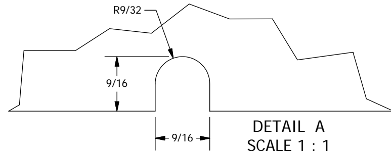
PFS03016 Insulation Frame Horizontal Long - Roof Quantity: 2
