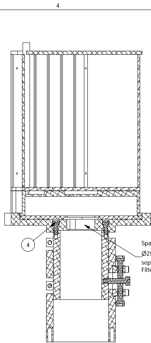
SECTION B-B
